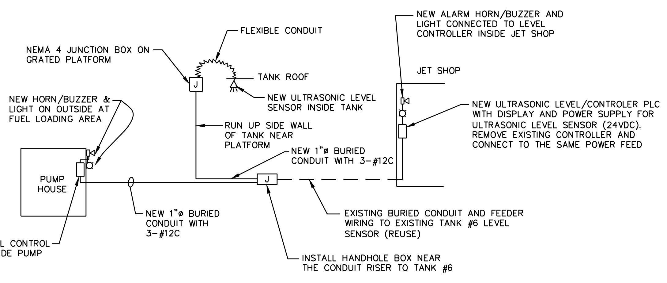
TANK LEVEL SENSING & ALARM LAYOUT
