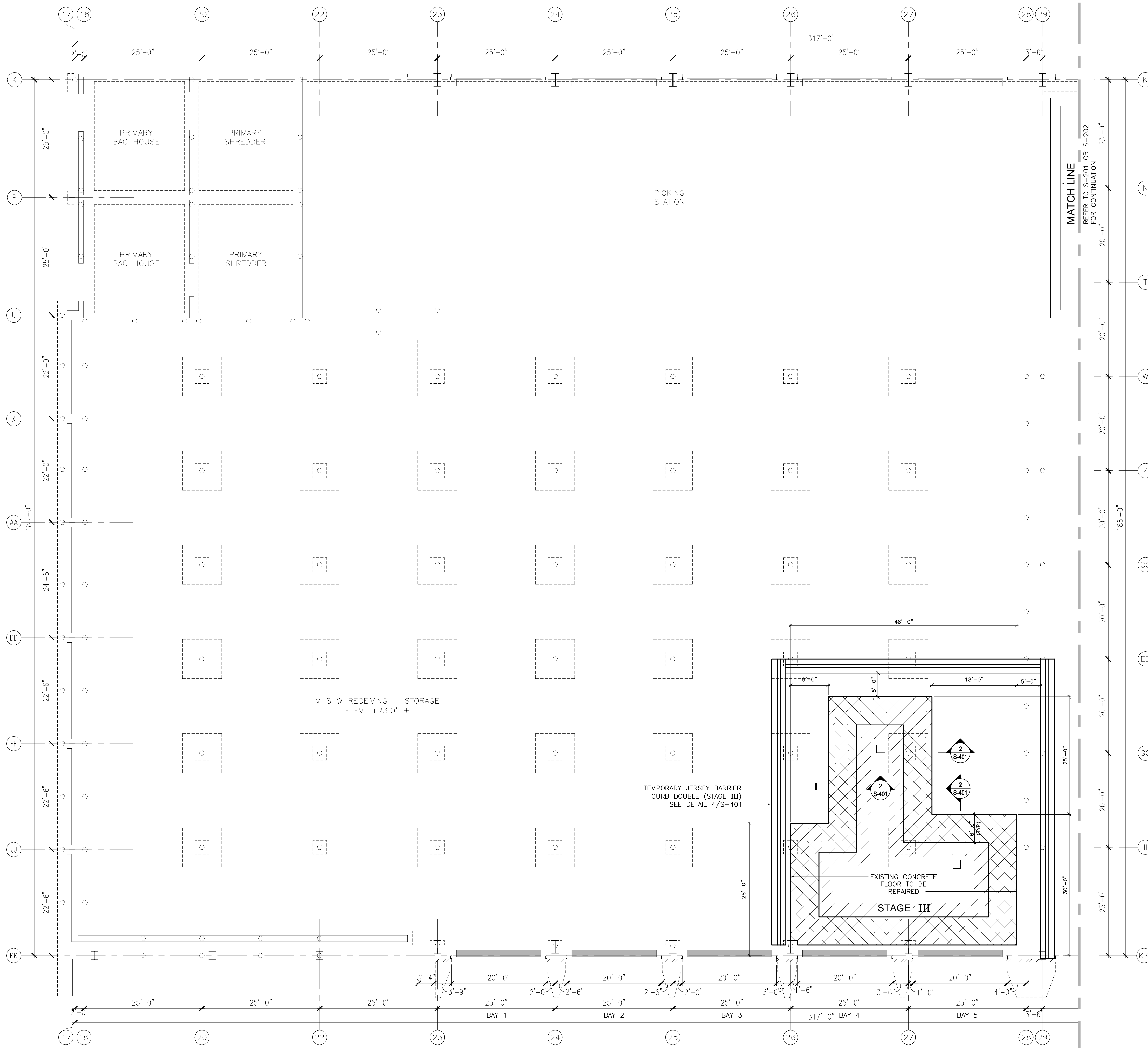
1 MSW FLOOR CONCRETE SLAB REPAIR PLAN (STAGE III) S-203
